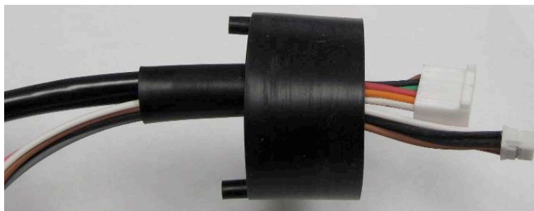
Figure 1. Insert Harnesses
